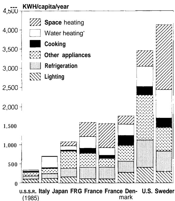
Figure 34—Home Electricity Use in 1986 U.S.S.R. and OECD Countries
