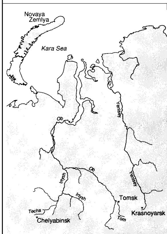
FIGURE 1-5: The Ob and Yenisey Rivers
