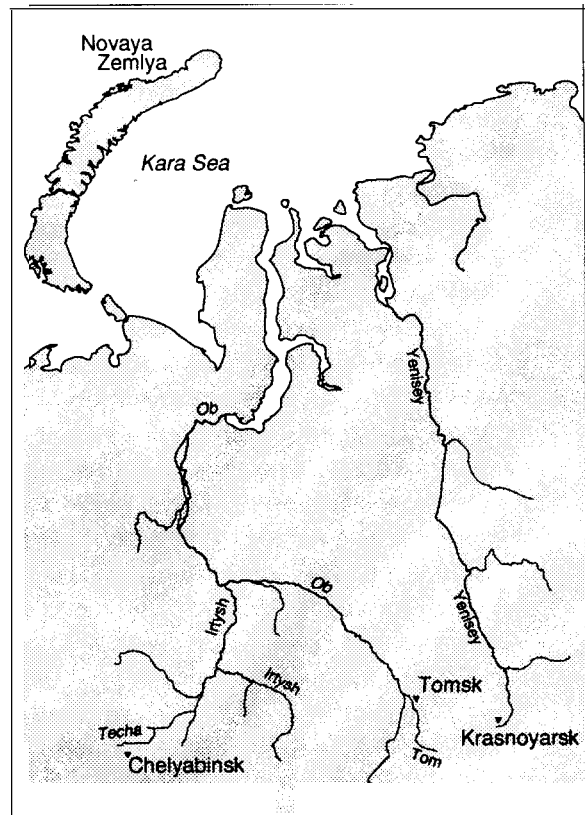
FIGURE 2-2: The Ob and Yenisey Rivers
