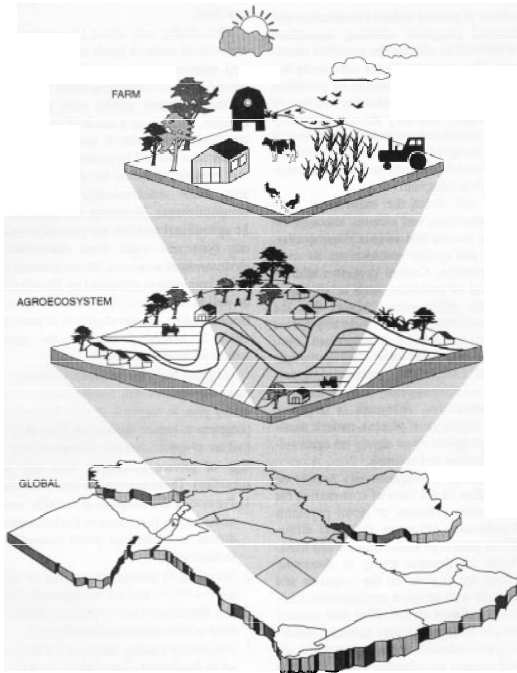
FIGURE 5: Agroecosystem
