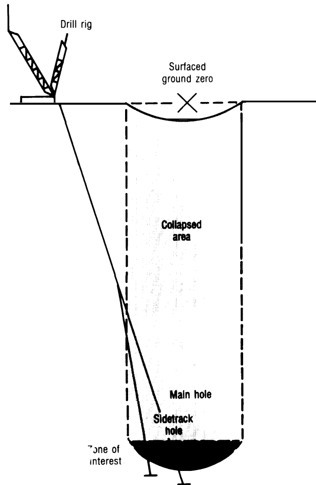
Figure 2-3-Drill-Back operation
