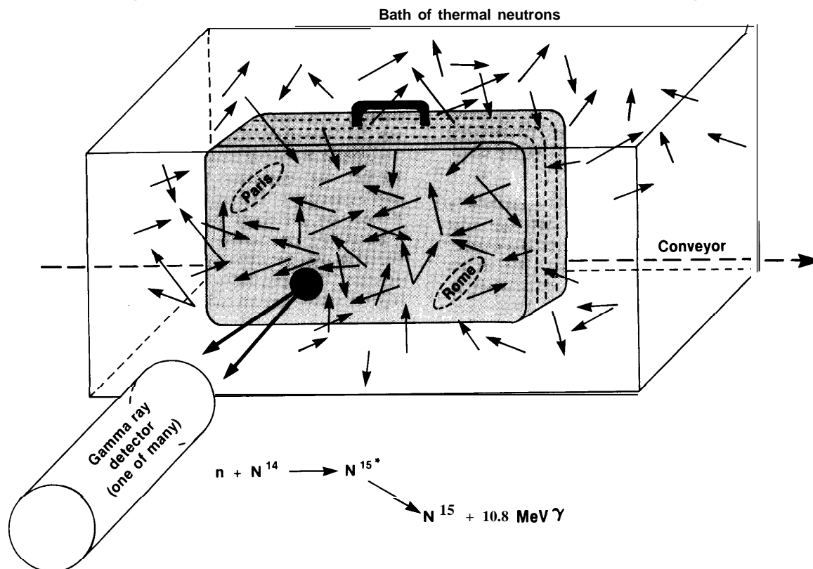
Figure A-1—Sketch of Apparatus for Thermal Neutron Analysis of Nitrogen
