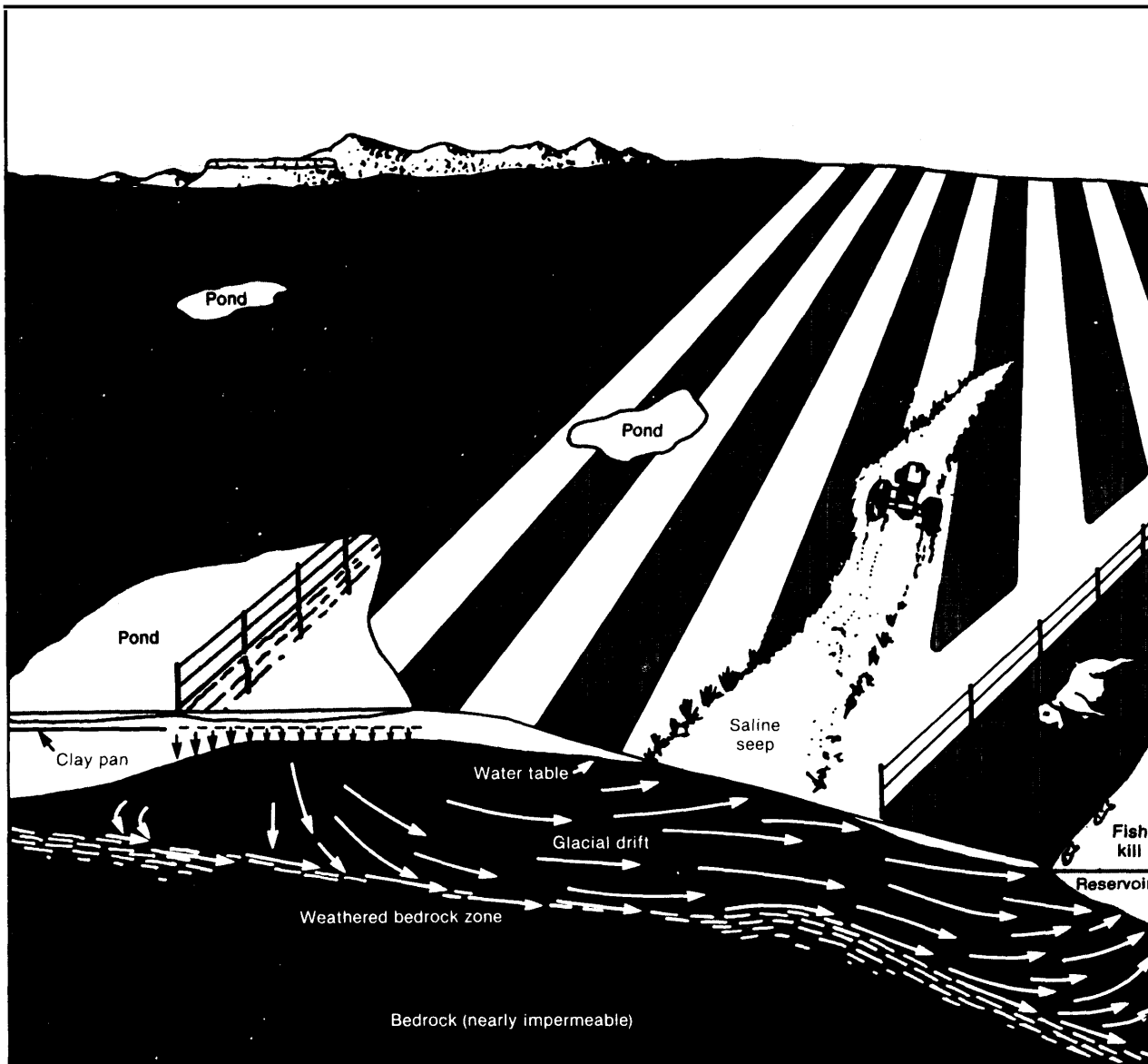
Figure 49. - Development of a Saline Seep
